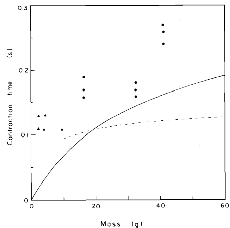
FIG. 16. Contraction time is plotted against body size (mass in grams) using data from T. L. Daniel (in preparation) for Gonionemus vertens (▲); Gladfelter (1973) for Liriope tetraphylla , Stomatoca atra , and Phialidium hemisphericum (●); and Spencer and Satterlie (1981) for Polyorchis penicillatus (broken line obtained from regression of author's data). The solid line in this figure represents the predicted mass which maximizes \eta/C for any contraction time.
