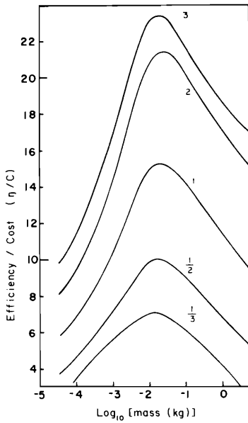
FIG. 14. The efficiency to cost ratio ( \eta/C ) is plotted against body mass for medusae of a variety of shapes with contraction phases lasting 0.1 s. Shape is specified above each line by a number equal to the ratio of bell height to radius. The mass which maximizes \eta/C is dependent of shape.
